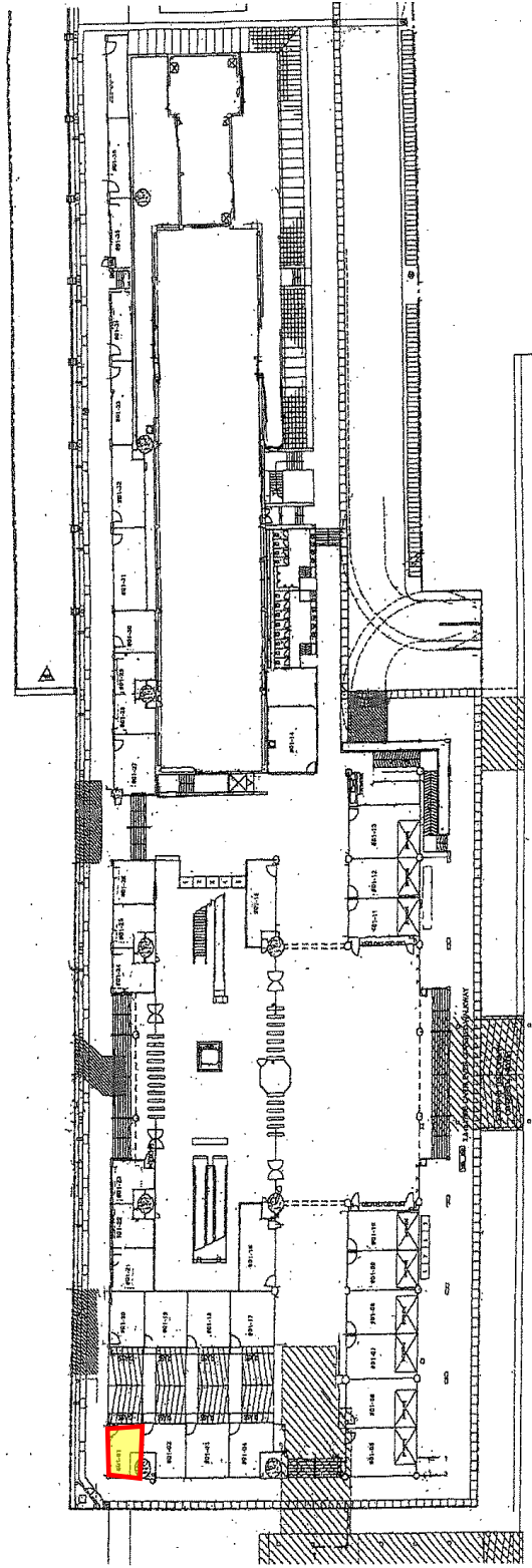
CONCOURSE LEVEL PLAN – BOON LAY MRT STATION (Floor Plan and Area Subject to changes)
