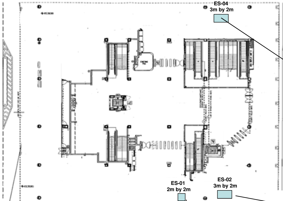
CONCOURSE LEVEL PLAN - BISHAN MRT STATION (FLOOR PLAN AND AREA -
